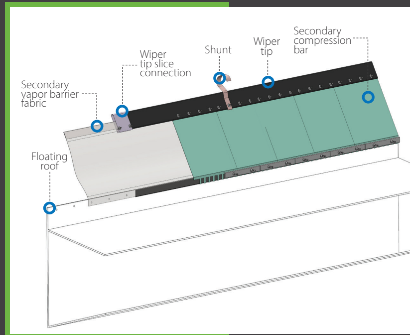
DirectFlex Secondary Metallic Wiper Seal
